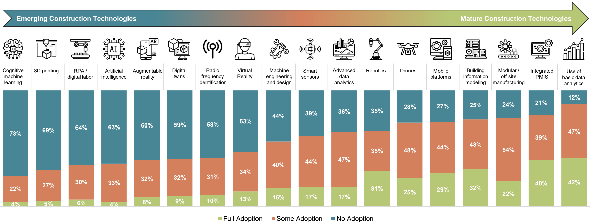
Construction Technologies Ranked By Current Adoption Level
